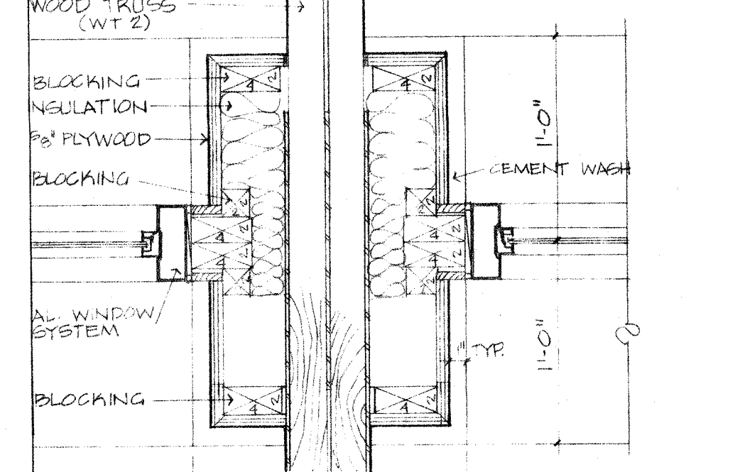
16 A10 PLAN OF TRUSS (WT 2) AT TOP OF MASONRY PIER SCALE 1/2\"/>
