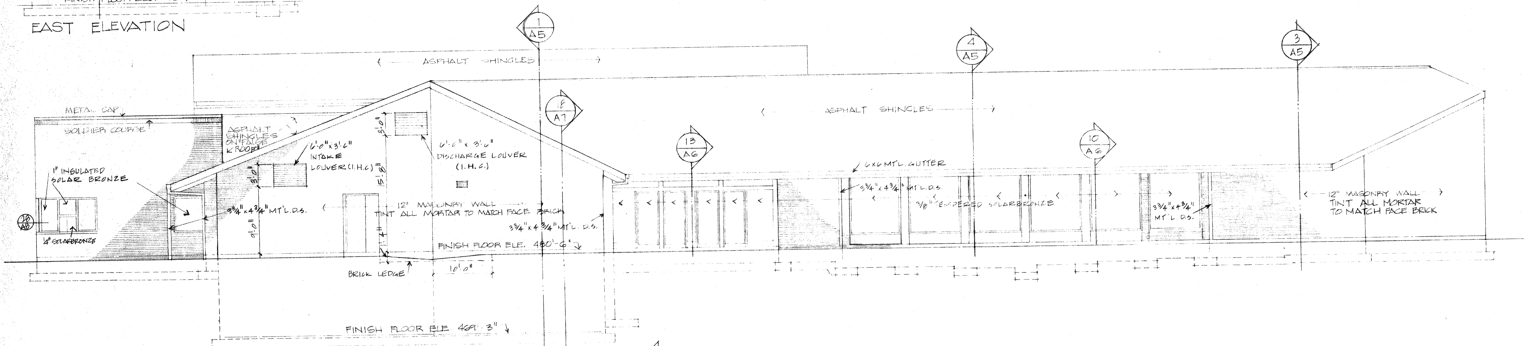
SOUTH ELEVATION
