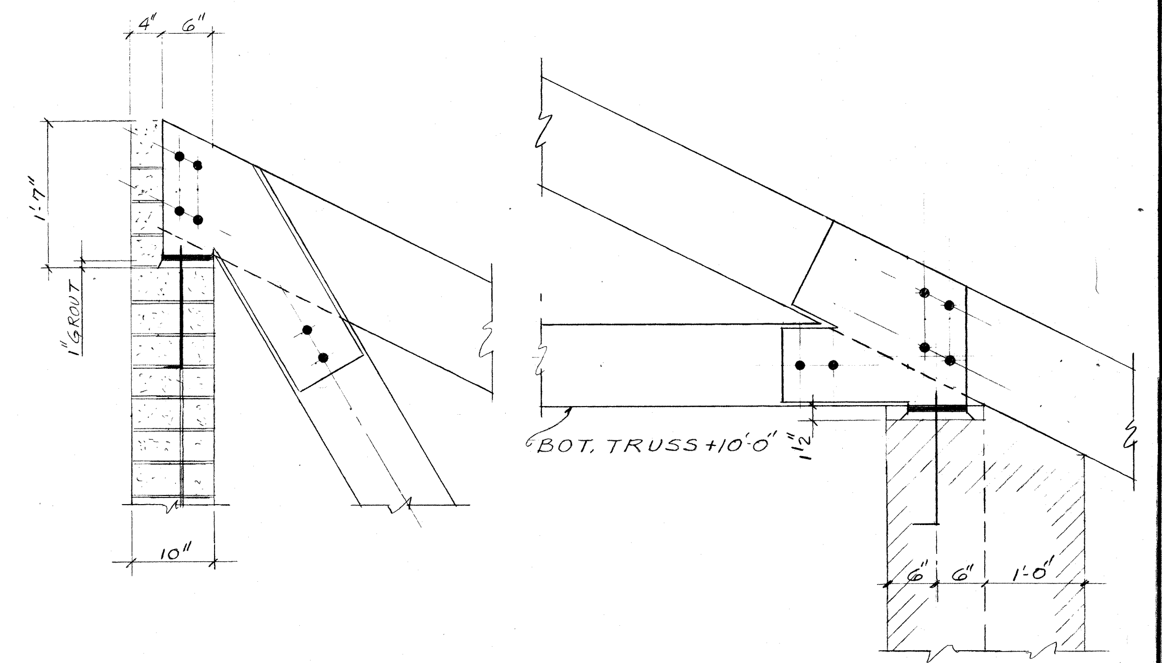
CONNECTION "A"
