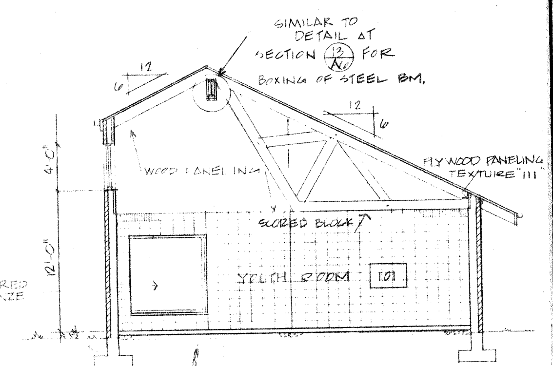
2 BUILDING SECTION
