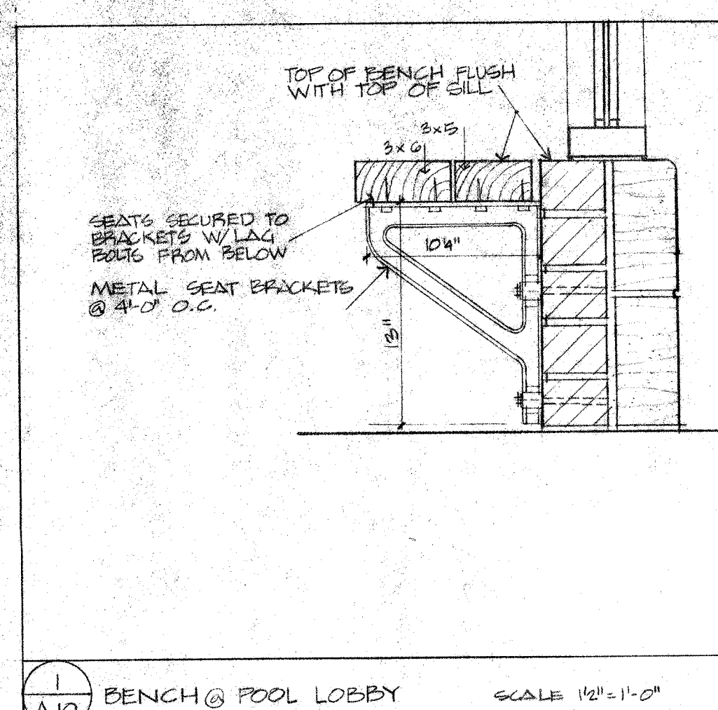
1 A10 BENCH @ POOL LOBBY SCALE 1/2\"/>
