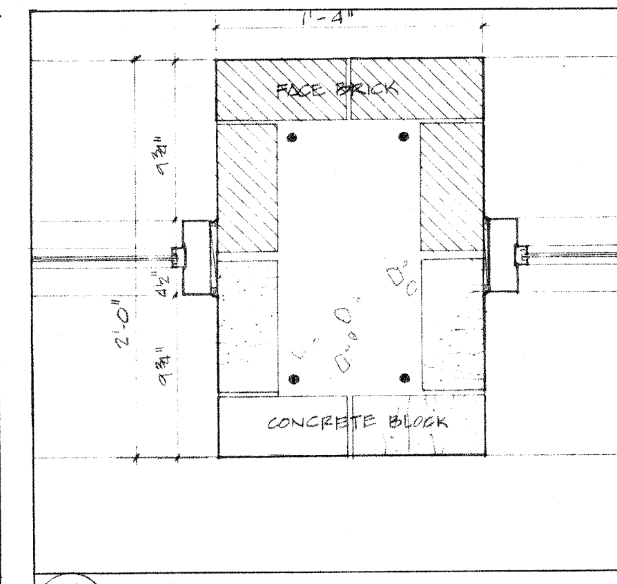
21 A10 PLAN OF MASONRY PIERS SCALE 1/2\"/>
