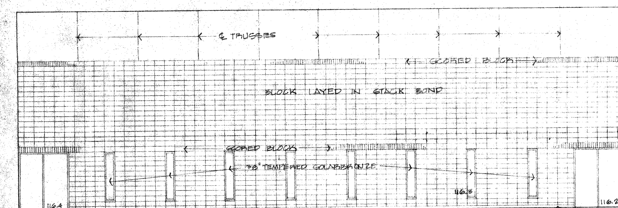
13 A10 MULTI-PURPOSE ROOM 116 NORTH WALL SCALE 1/2\"/>
