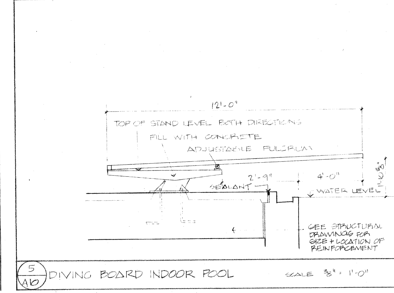
5 A10 DIVING BOARD INDOOR POOL SCALE 3/8\"/>
