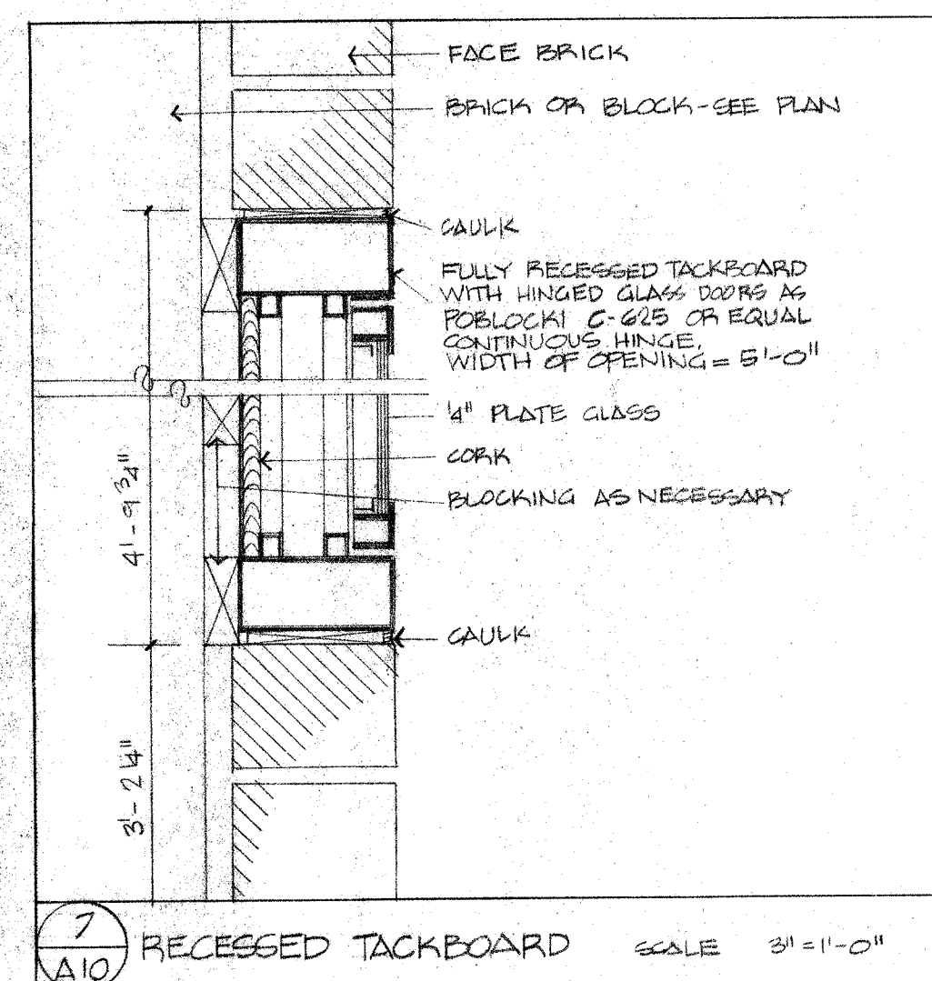
7 A10 RECESSED TACKBOARD SCALE 3/4\"/>
