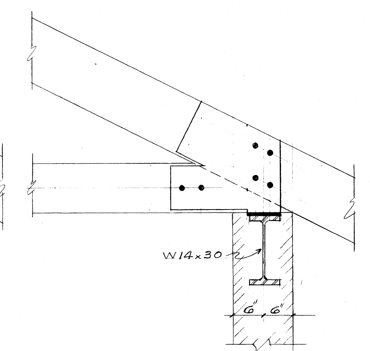
SECTION 2
