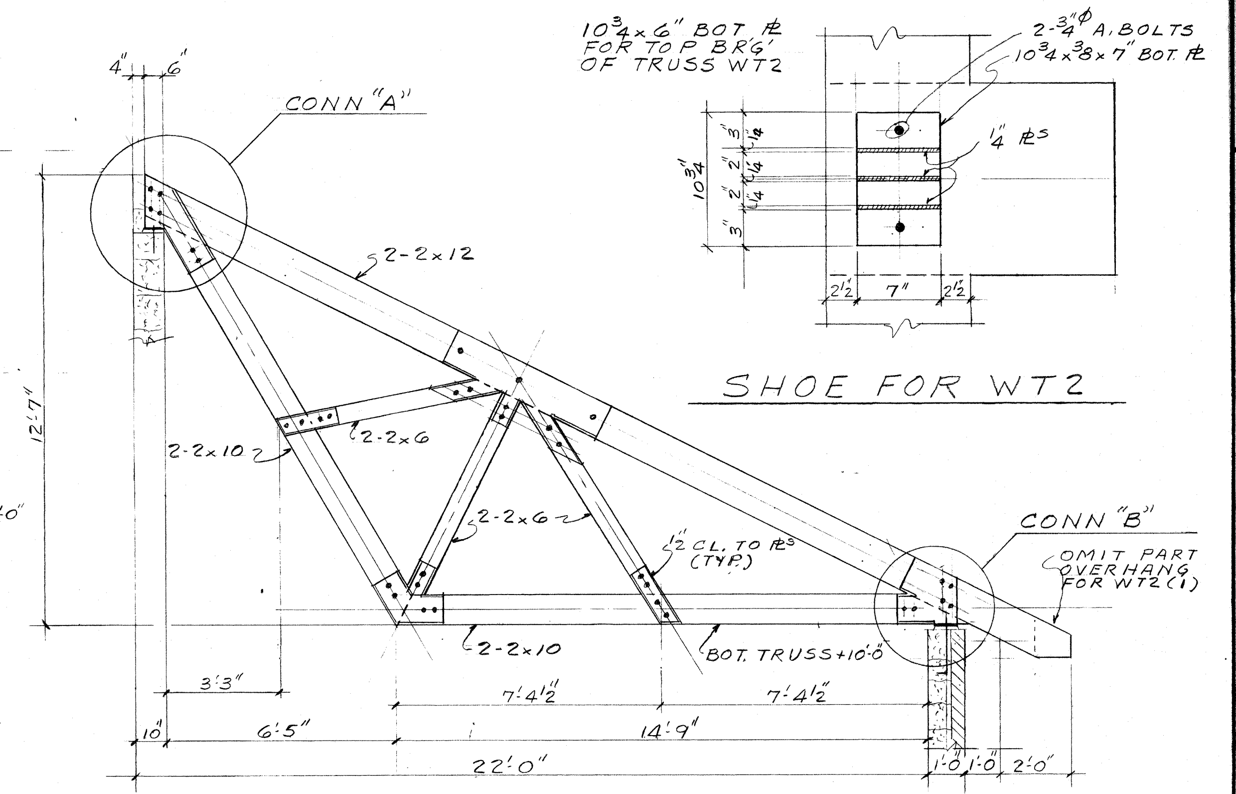
WOOD TRUSS (WT2) SCALE: 3/8"=1'-0"
