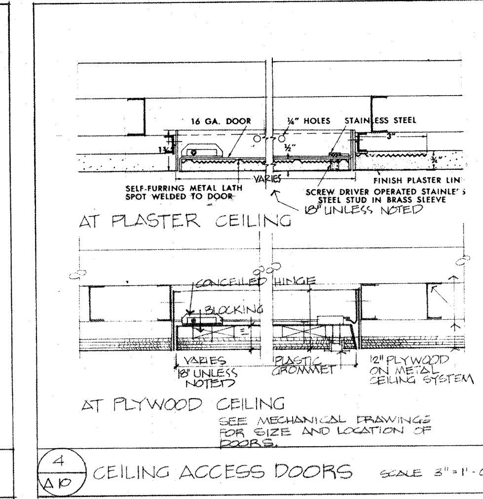
4 A10 CEILING ACCESS DOORS SCALE 3/4\"/>
