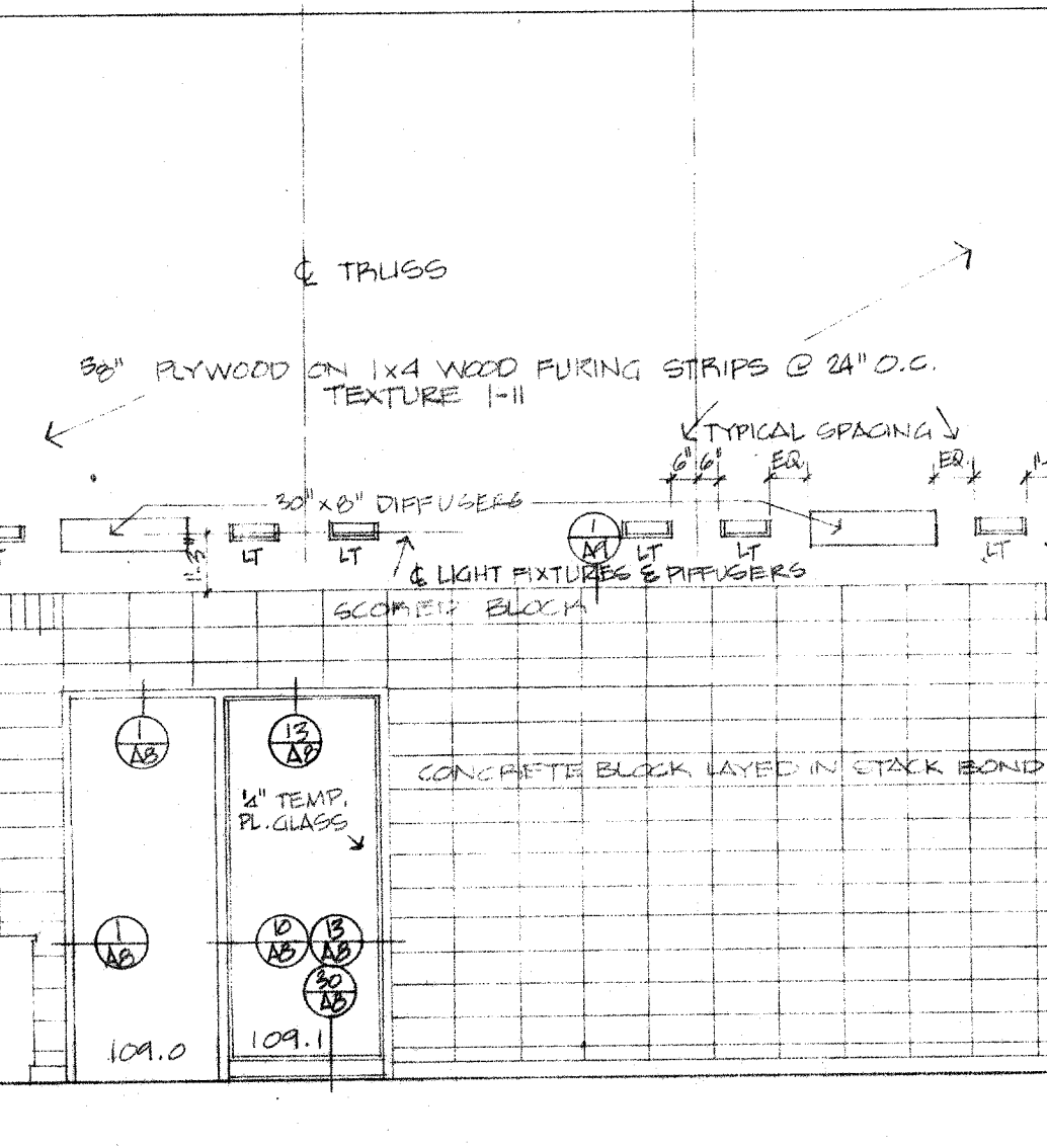
23 A10 LIGHT FIXTURES & DIFFUSERS ROOM 105 SCALE 1/4\"/>
