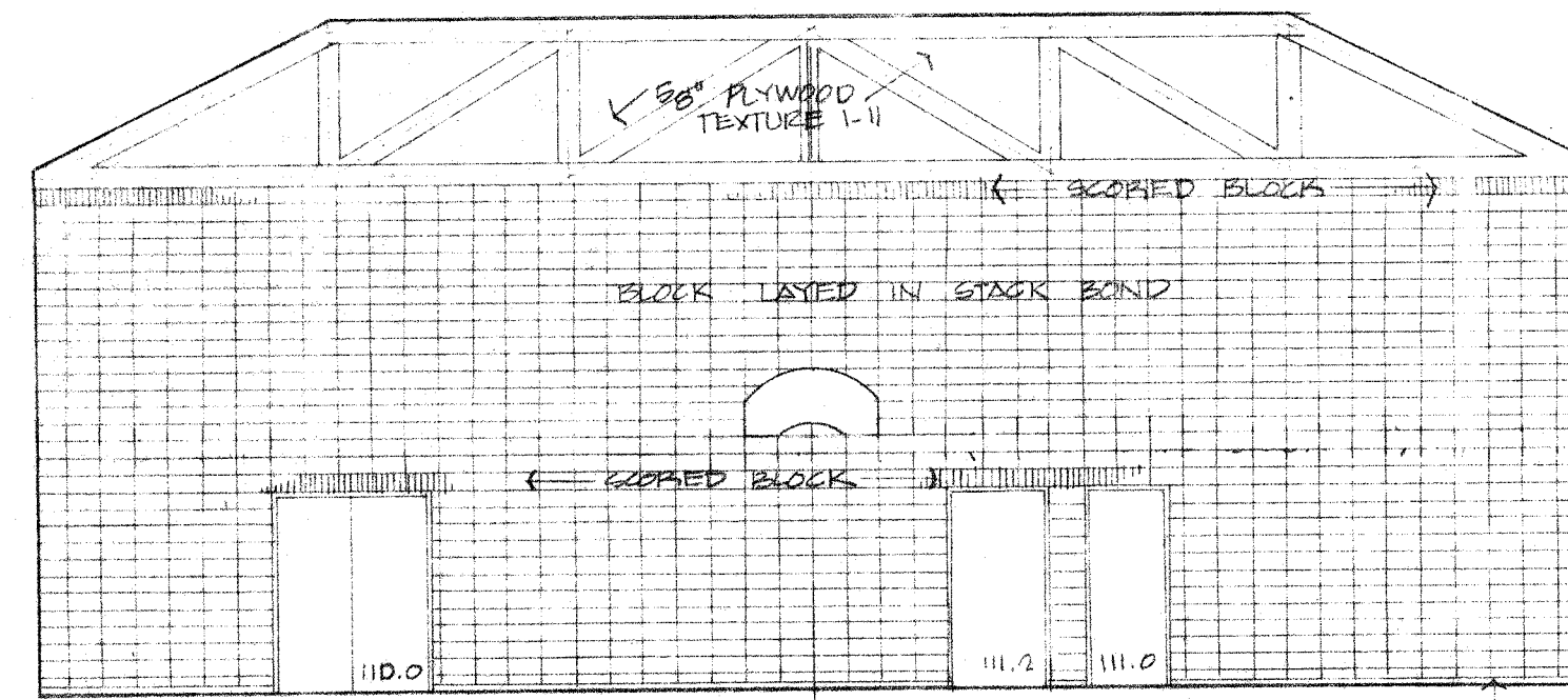
14 A10 MULTI-PURPOSE ROOM 116 EAST WALL SCALE 1/2\"/>
