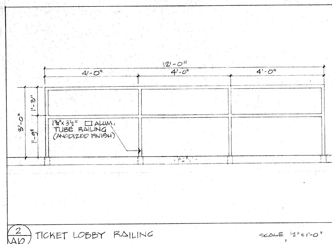
2 A10 TICKET LOBBY RAILING SCALE 1/2\"/>
