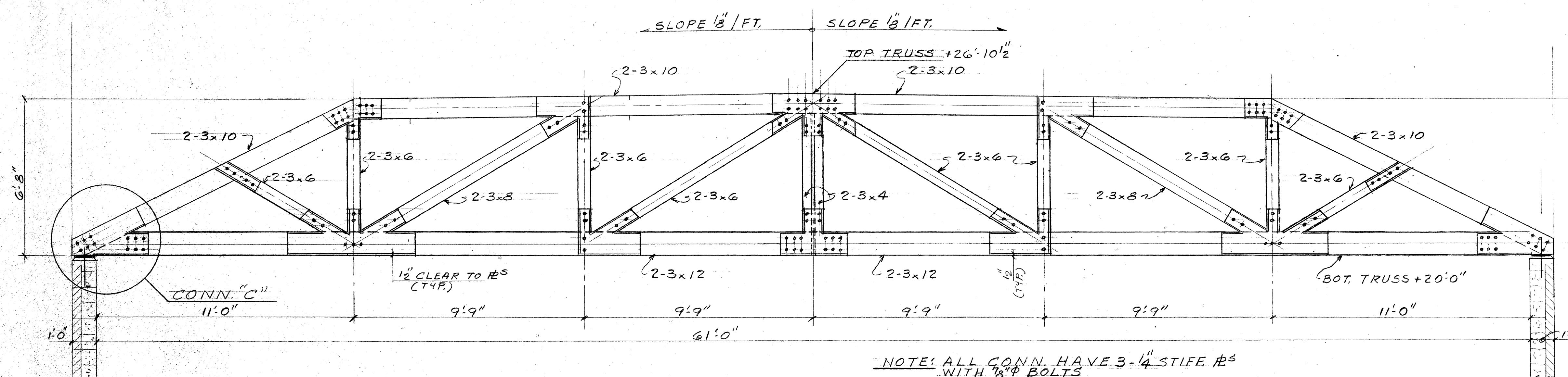
WOOD TRUSS (WT1) SCALE: 3/8"=1'-0"
