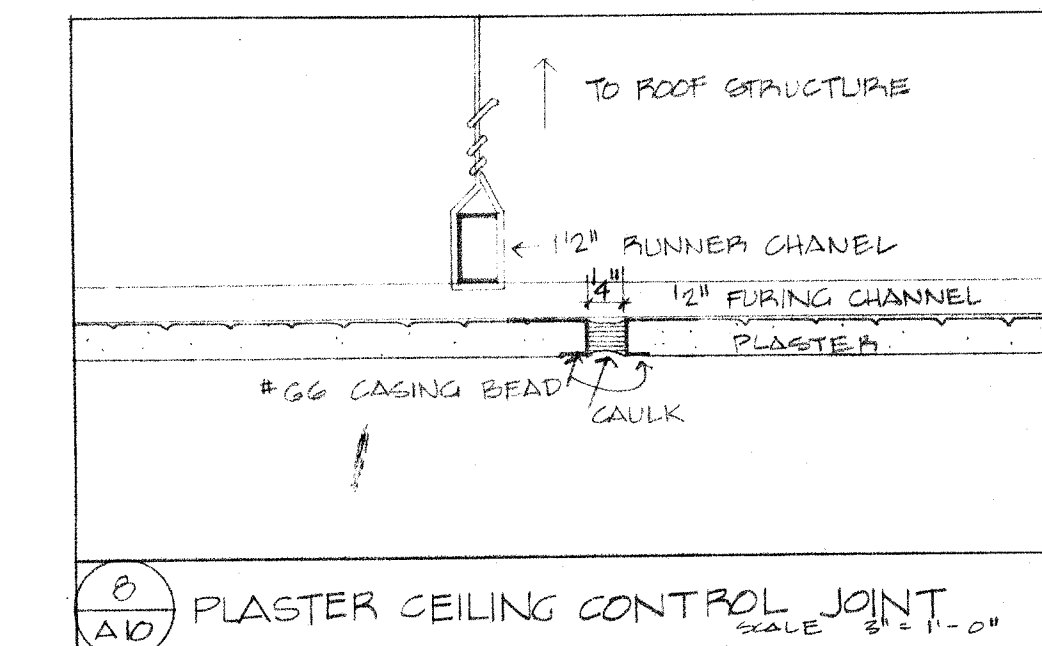
8 A10 PLASTER CEILING CONTROL JOINT SCALE 3/4\"/>
