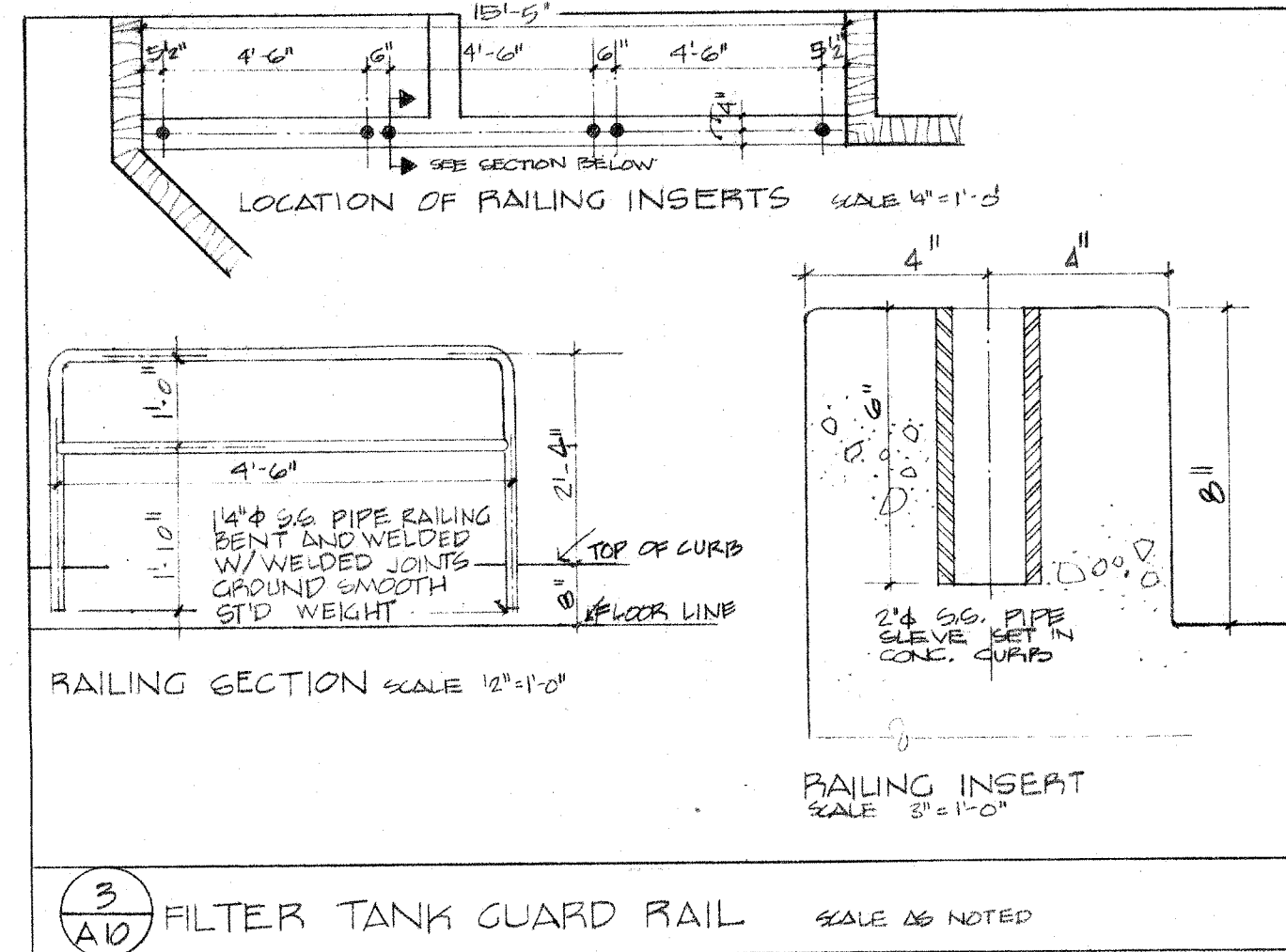
3 A10 FILTER TANK GUARD RAIL SCALE AS NOTED
