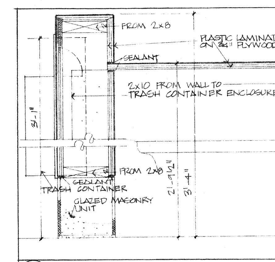
12 A10 TRASH CONTAINER ENCLOSURE SCALE 1/2\"/>
