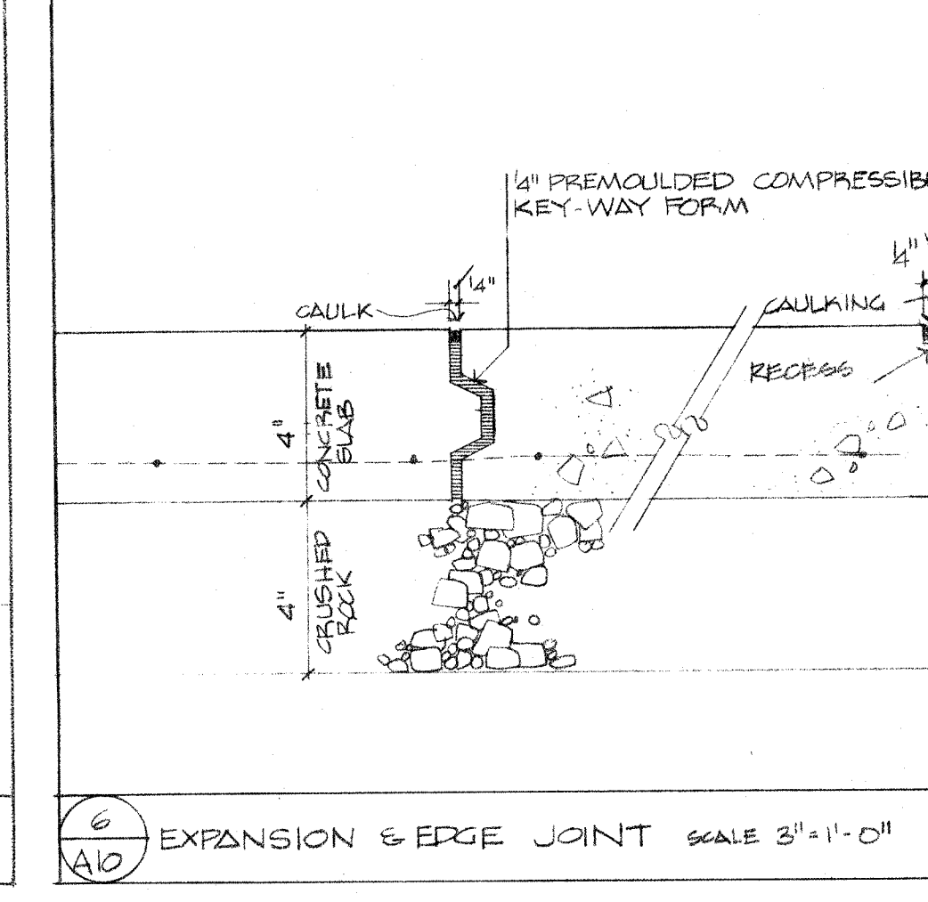
6 A10 EXPANSION & EDGE JOINT SCALE 3/4\"/>
