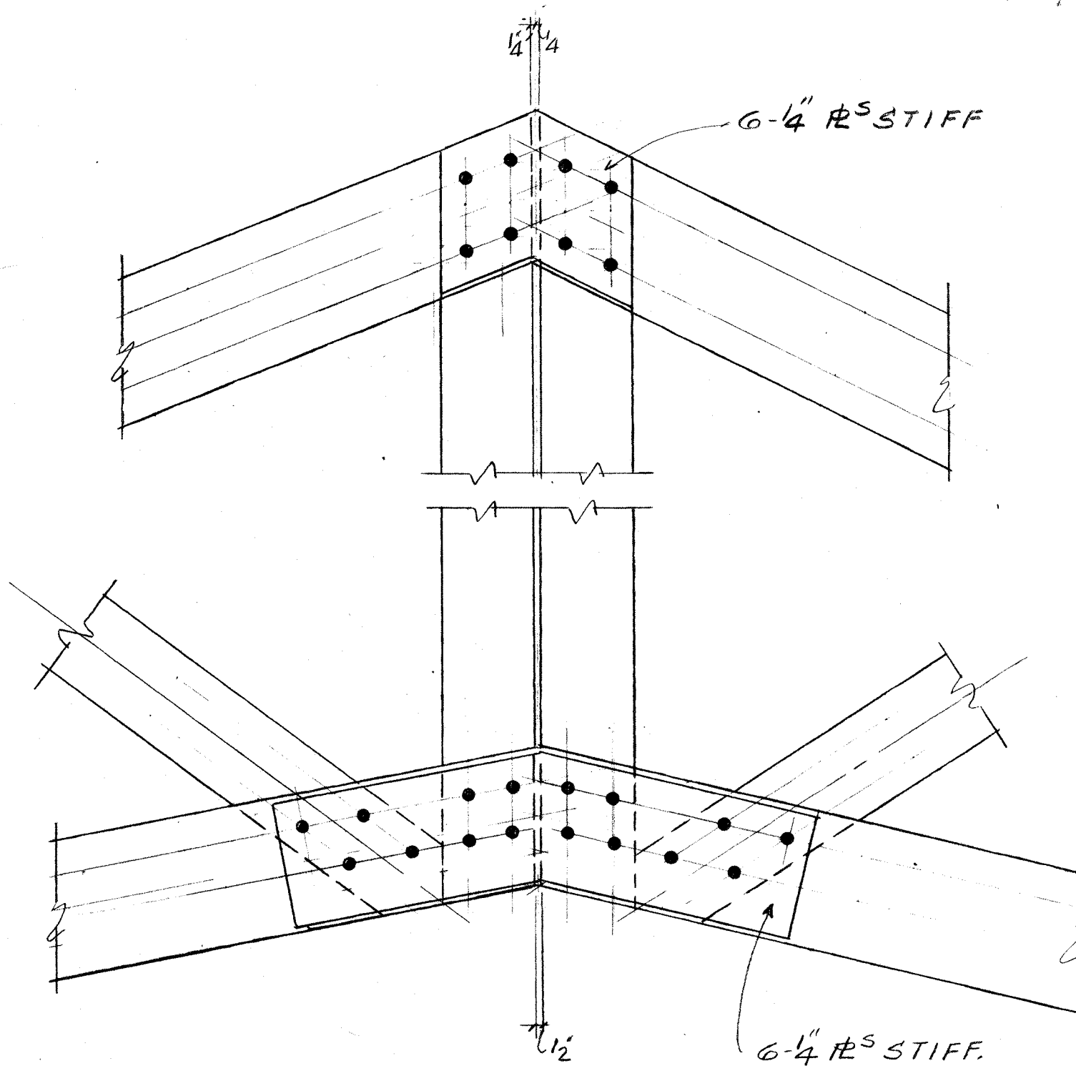
CENTER CONNECTION WT3
