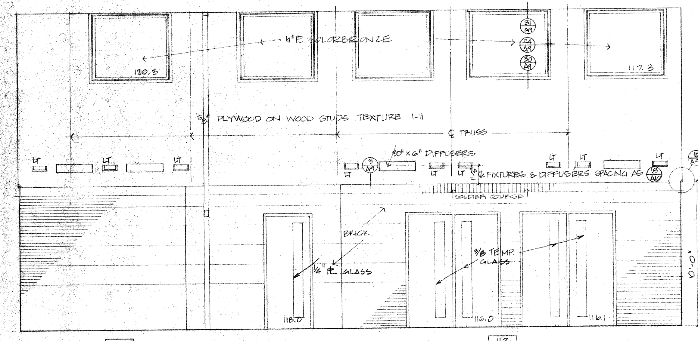
13 A10 MULTI-PURPOSE ROOM 116 NORTH WALL SCALE 1/2\"/>
