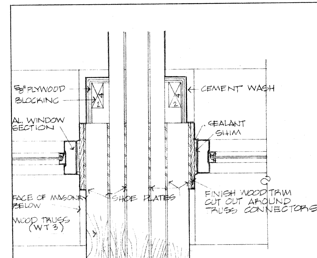
12 A10 PLAN OF TRUSS (WT 3) AT TOP OF MASONRY PIER SCALE 1/2\"/>
